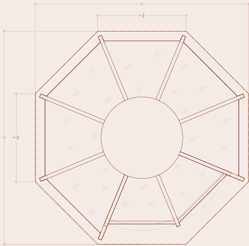
GENERAL VIEW - TOP W/ DOOR
