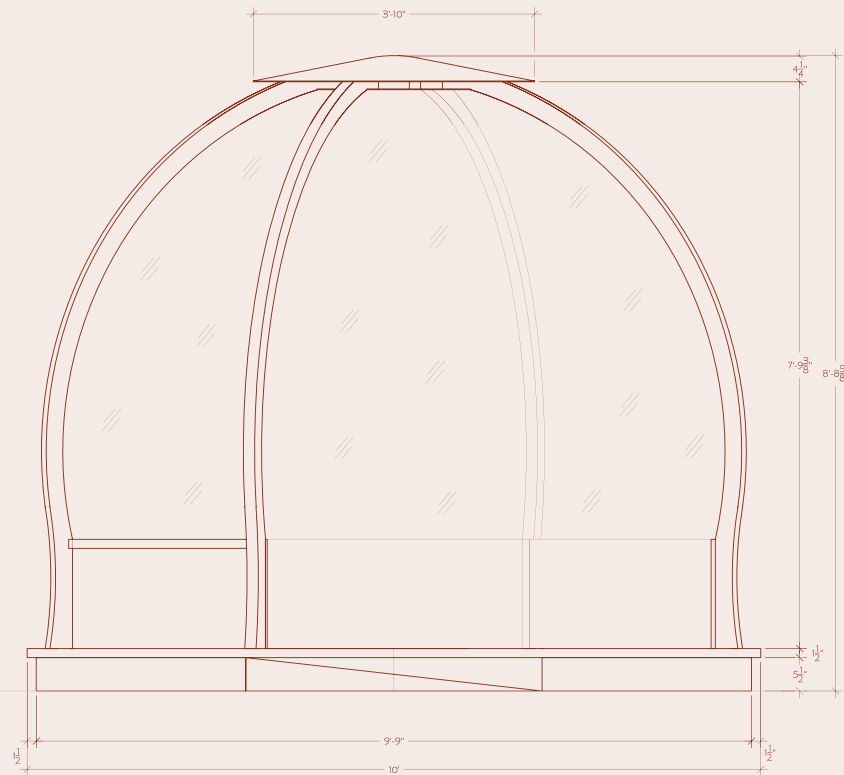
GENERAL VIEW - ELEVATION W/O DOOR
